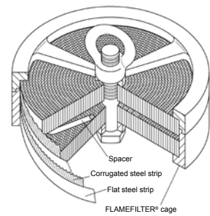
Figure 6: Extinguishing the flame in the narrow gap (flame quenching) by heat transfer
