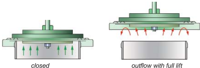
Fig. 1: Outflow with a full-lift disc and air cushion seal
