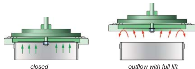
Fig. 2: Outflow with a full-lift disc and metal seal
